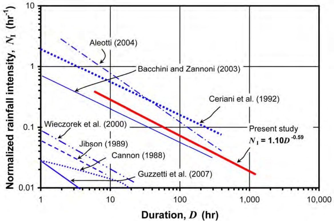
Fig. 10. Comparison of the normalized rainfall intensity–duration thresholds from various studies.
