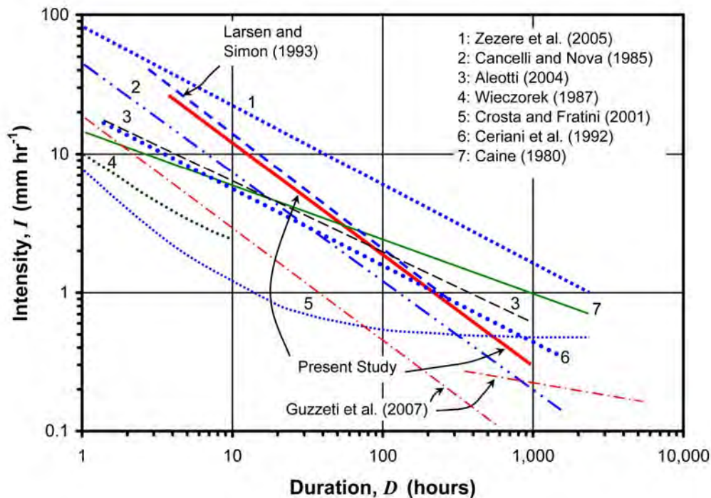
Fig. 9. Comparison of the landslide triggering rainfall intensity–duration thresholds from various studies.
