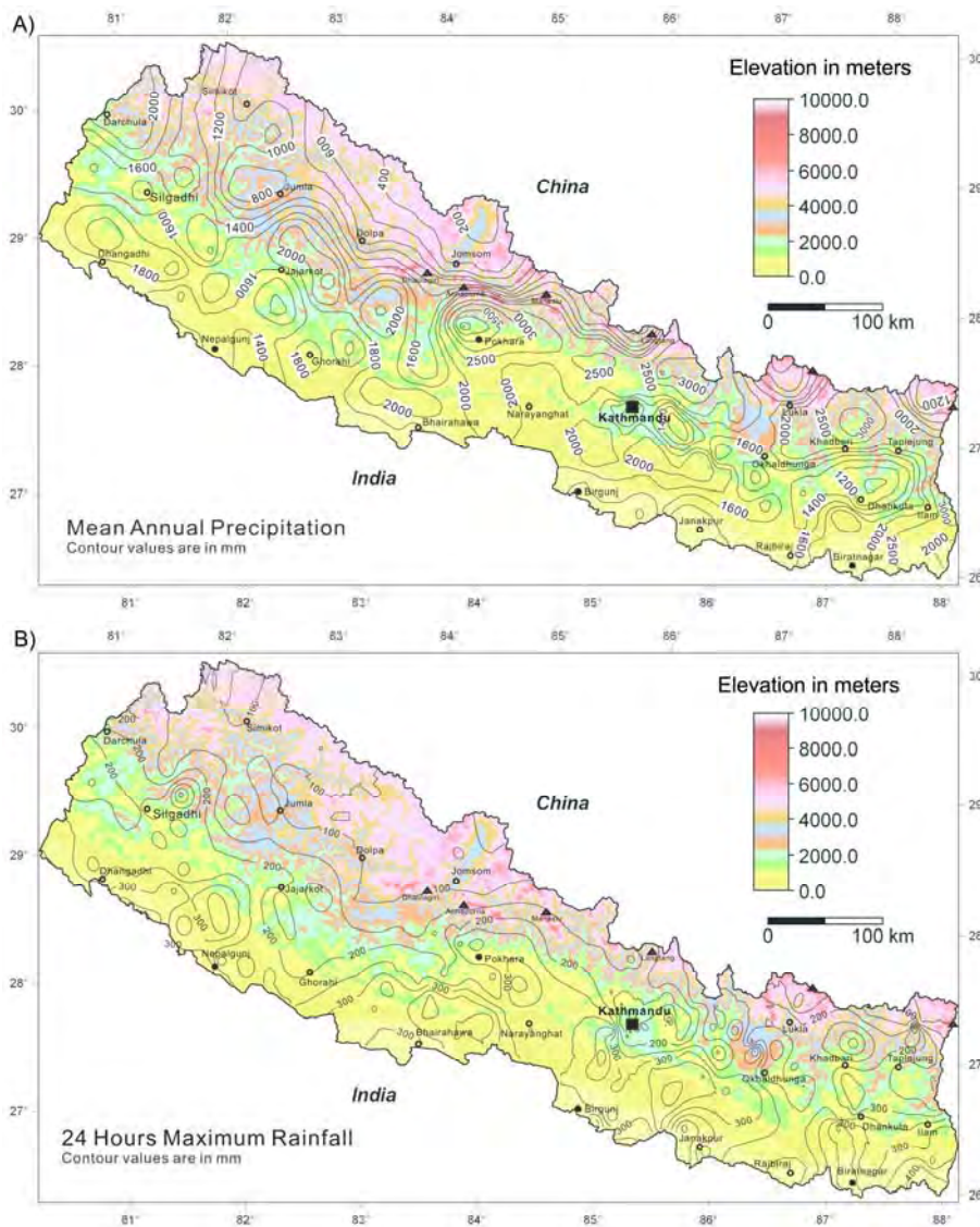
Fig. 3. Rainfall distribution in Nepal. A) Mean annual precipitation; B) Maximum rainfall of 24 hours. In both figures peak values are around central Nepal (modified after DHM, 2000, 2003).
