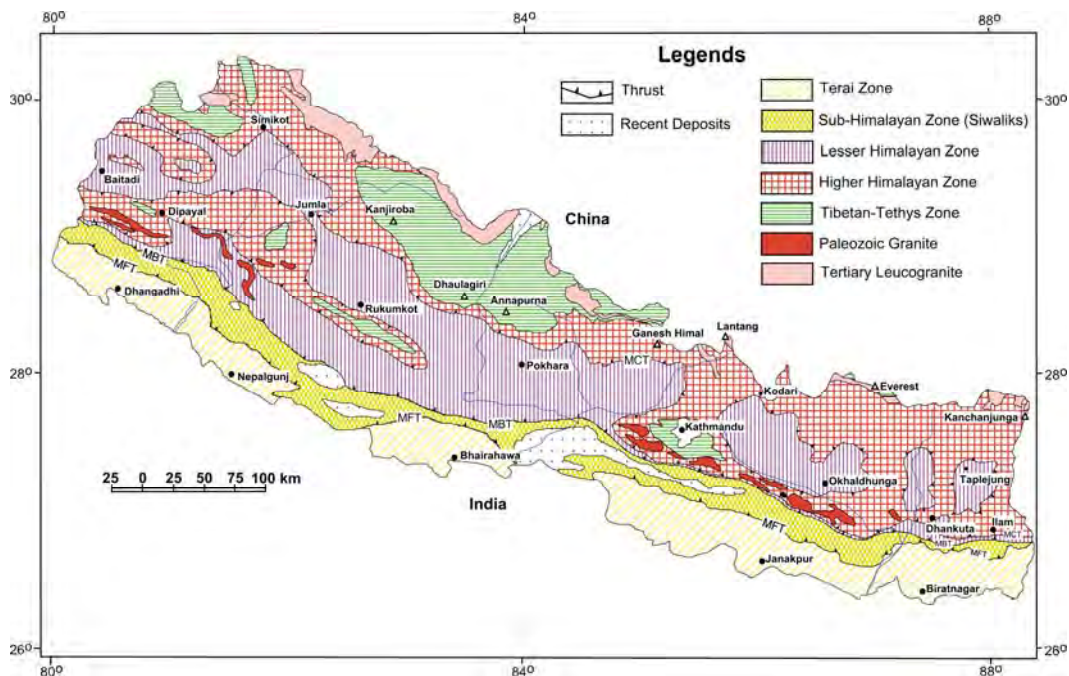
Fig. 2. Geological map of Nepal (modified after Amatya and Jnawali, 1994; Dahal, 2006c)
