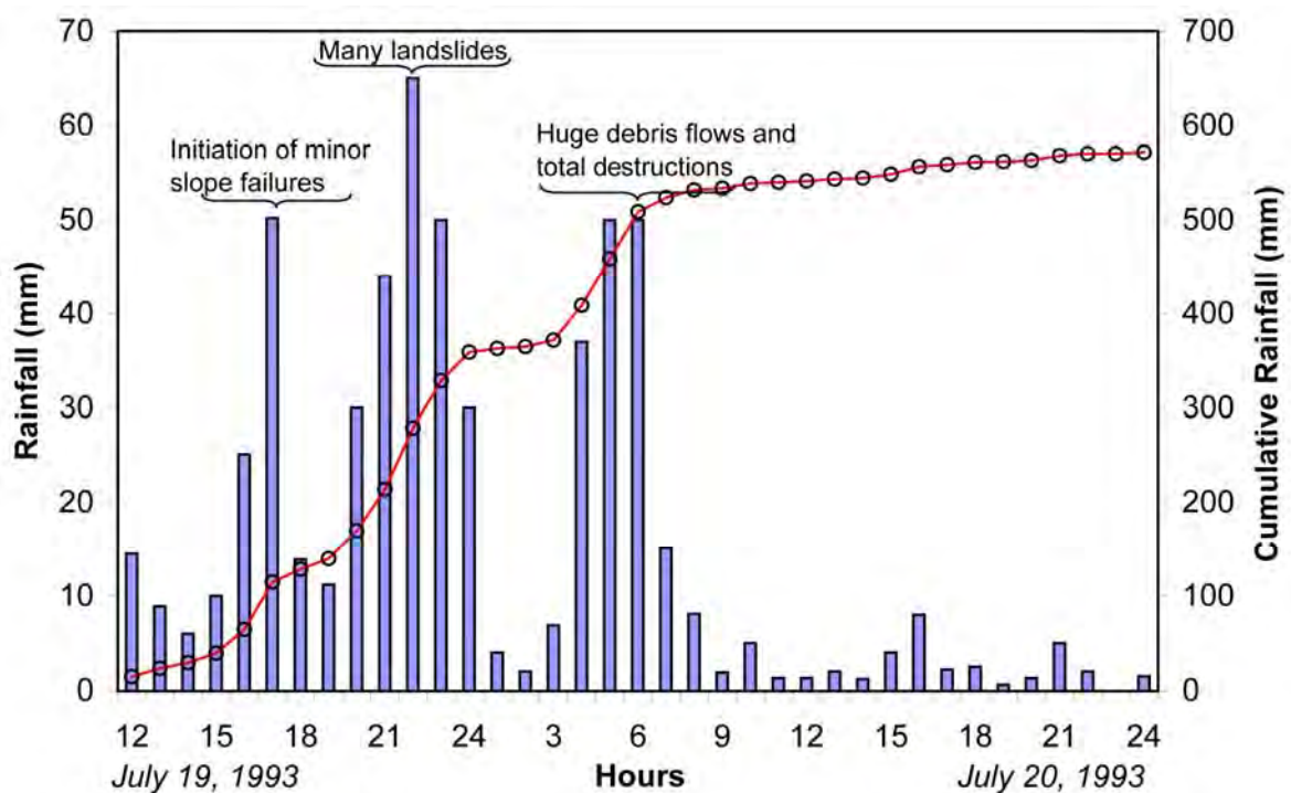
Fig. 7. Rainfall at Tistung, central Nepal on July 19 and 20, 1993, and the landslides disaster associated with this extreme rainfall, the highest one day precipitation (541.4 mm) ever recorded in Nepal (source: Department of Soil Conservation and Watershed Management)
