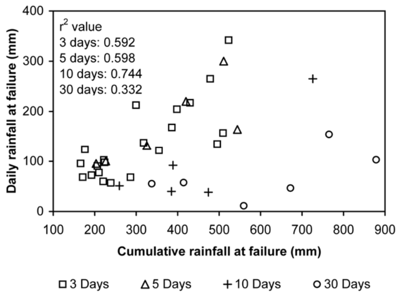
Fig. 12. Relationships between daily rainfall at failure and total rainfall of monsoon at failure, with correlation coefficient values.
