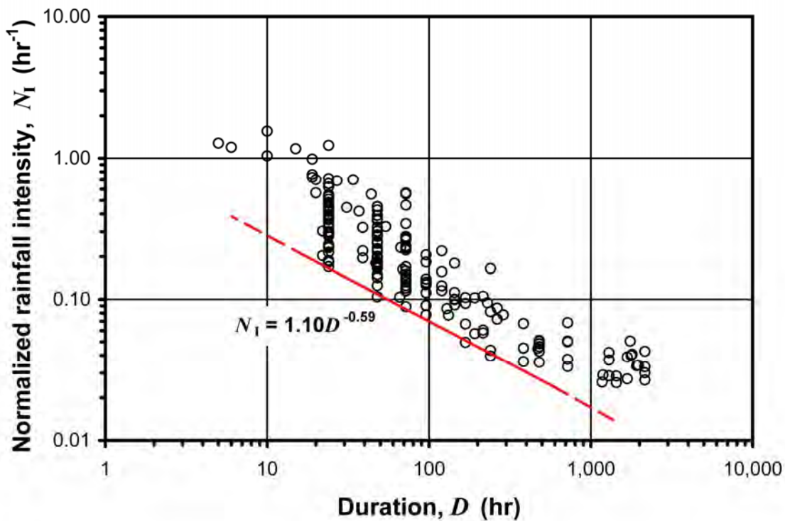
Fig. 8. Normalized rainfall intensity–duration thresholds for the initiation of landslides in the Nepal Himalaya.
